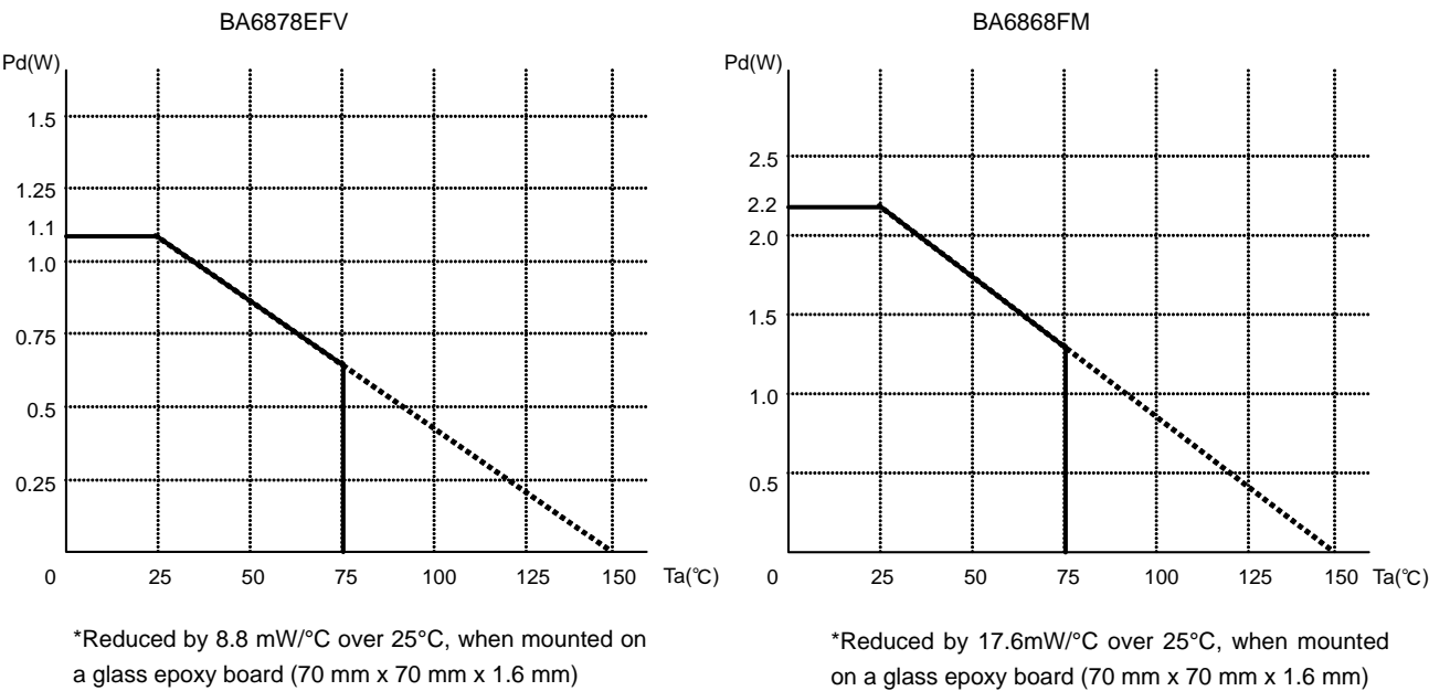
Fig.38 Heat Derating Curve
